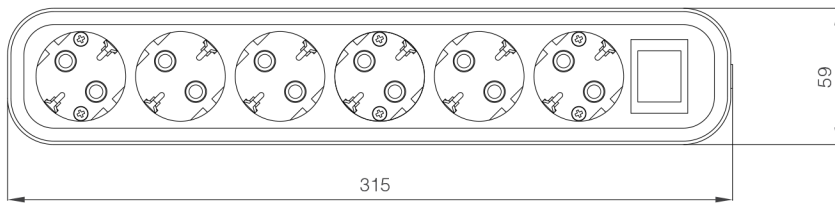
6 Gang Earthed Socket with Switch
