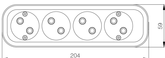
4 Gang Socket without Earthed
