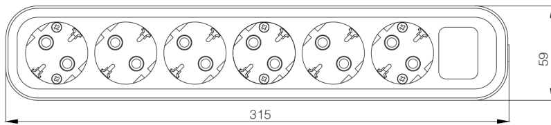
6 Gang Earthed Socket
