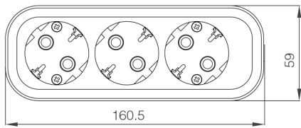
3 Gang Earthed Socket
