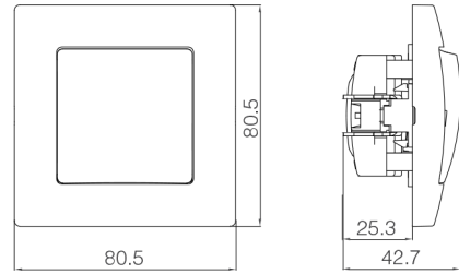
One Way Switch
