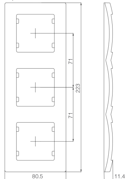
Triple Vertical Frame
