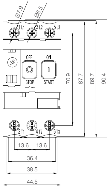
Motor Protection Breaker
