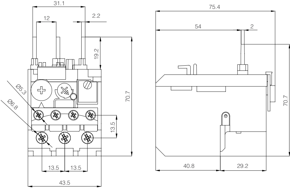
Thermal Relay 18A
