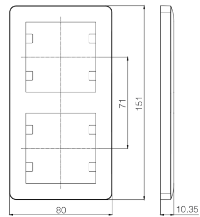
Double Vertical Frame
