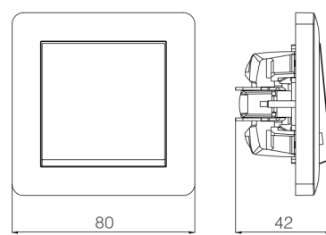
One Way Switch
