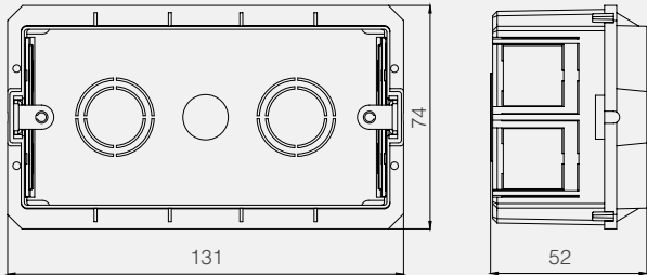
4M Flush Mounted Cases
