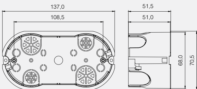
4M Cavity wall Case
