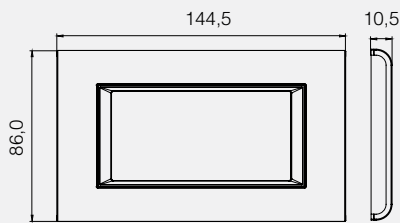
Cellia 4M Frame
