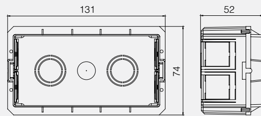
4 M Flush Mounted Cases
