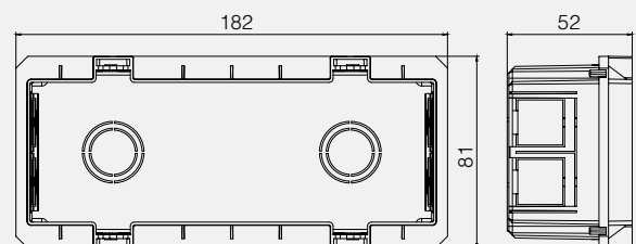
7 M Flush Mounted Cases
