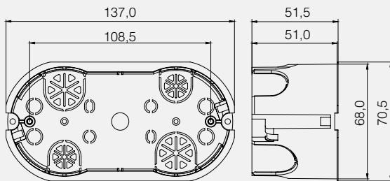
4M Cavity Wall Case
