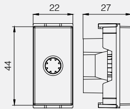
Cable Outlet Cover
