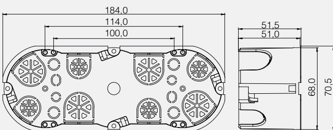
7 M Cavity Wall Case
