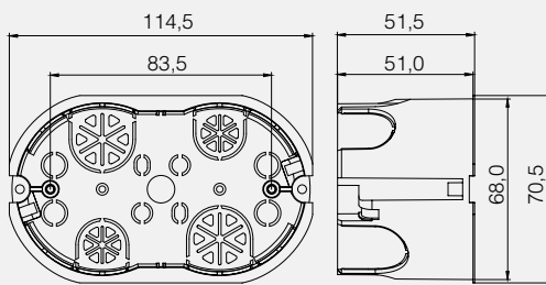
3M Cavity Wall Case
