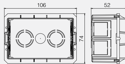
3 M Flush Mounted Cases
