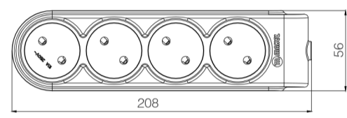
4 Gang Socket without Earthed
