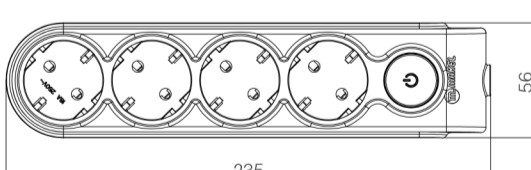
4 Gang Earthed Socket with Switch
