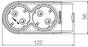
2 Gang Earthed Socket
