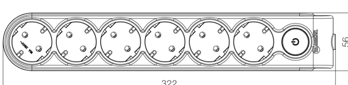
6 Gang Earthed Socket with Switch
