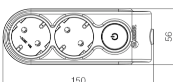
2 Gang Earthed Socket with Switch
