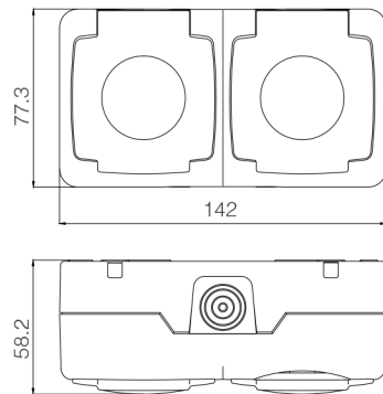
Double Schuko Socket Outlet With Cover
