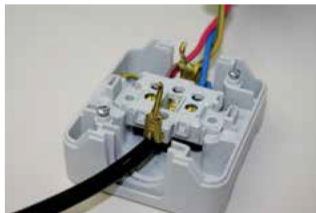
There are two options with or without screw terminals (quick connection)
