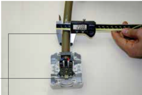
Conduits permit as Ø20 mm diameter. Mechanisms can fit own place tight.
