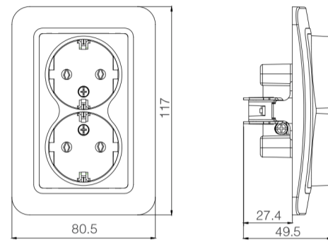
Double Schuko Socket Outlet
