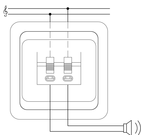
Loudspeaker - connection, 1 gang
