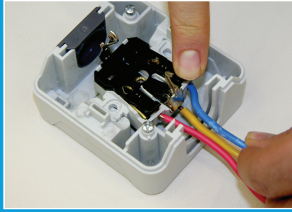
Soketli bağlantı Without screw terminals and socket-outlets
