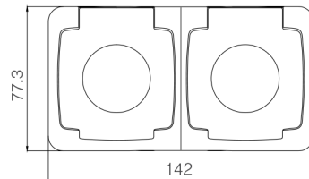
Double Schuko Socket Outlet With Cover
