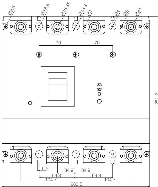
500 A, 630 A, 800 A Leak Current Protected Compact Switch
