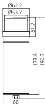
Tube Capacitor 4 (1,38 kVar)
