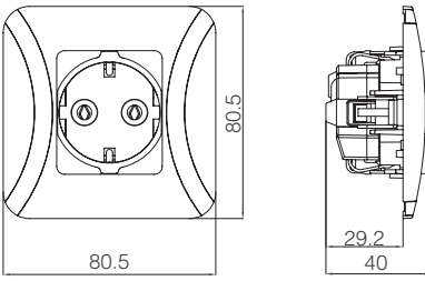
Topraklı Priz
