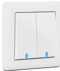
2G Change-Over Switch Illuminated BR011401 20 A - 16 AX, 250 V~ BS EN 60669-1
