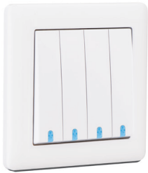
4G Switch Illuminated BR010801 20 A - 16 AX, 250 V~ BS EN 60669-1
